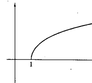
Fig. 4.13: y = \text{settcosh } x
