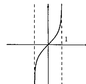
Fig. 4.14: y = \text{settanh } x
