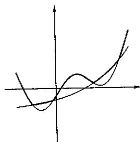
Fig. 4.35 : f \vee g = \max\{f, g\}
