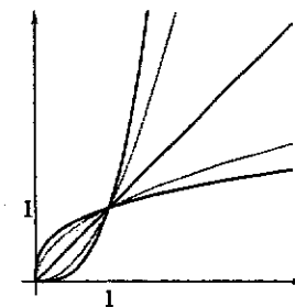
Fig. 1.6: y = x^3, x^2, x, \sqrt{x}, \sqrt[3]{x}
