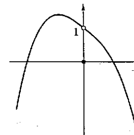
Fig. 6.3: f(0) = 0
