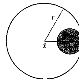
Fig. A4.6: B_{r'}(y) \subset B_r(x)
