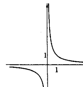
Fig. 1.8: y = 1/x
