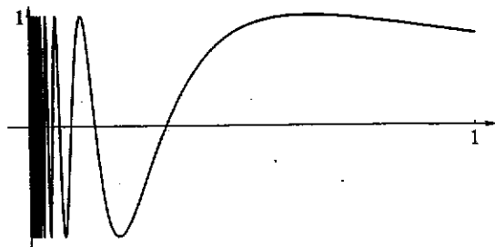
Fig. 6.4: y = \sin(1/x)
