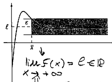
Fig. 6.1: \lim_{x \rightarrow +\infty} f(x) = \ell
