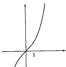
Fig. 4.9: y = \sinh x
