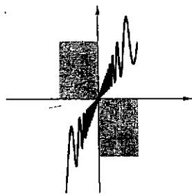
Fig. A4.2: y = 2x + x \text{sen}(1/x) per x \in [-0.1, 0.1]
